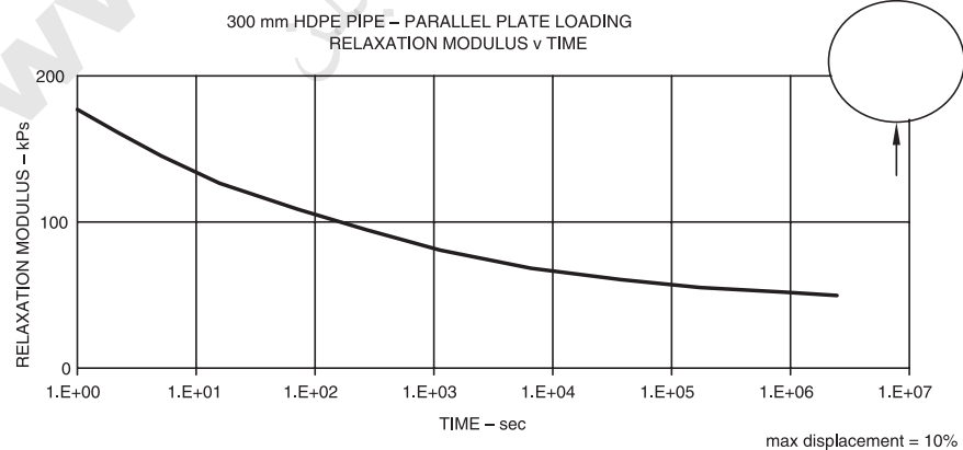
Figure 4-3: Stiffness Relaxation
