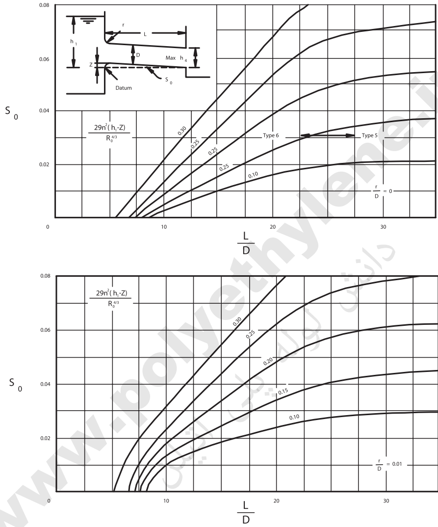
Figure 2-9: Circular Sections
