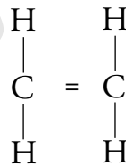
Figure 1-1b: Ethylene
